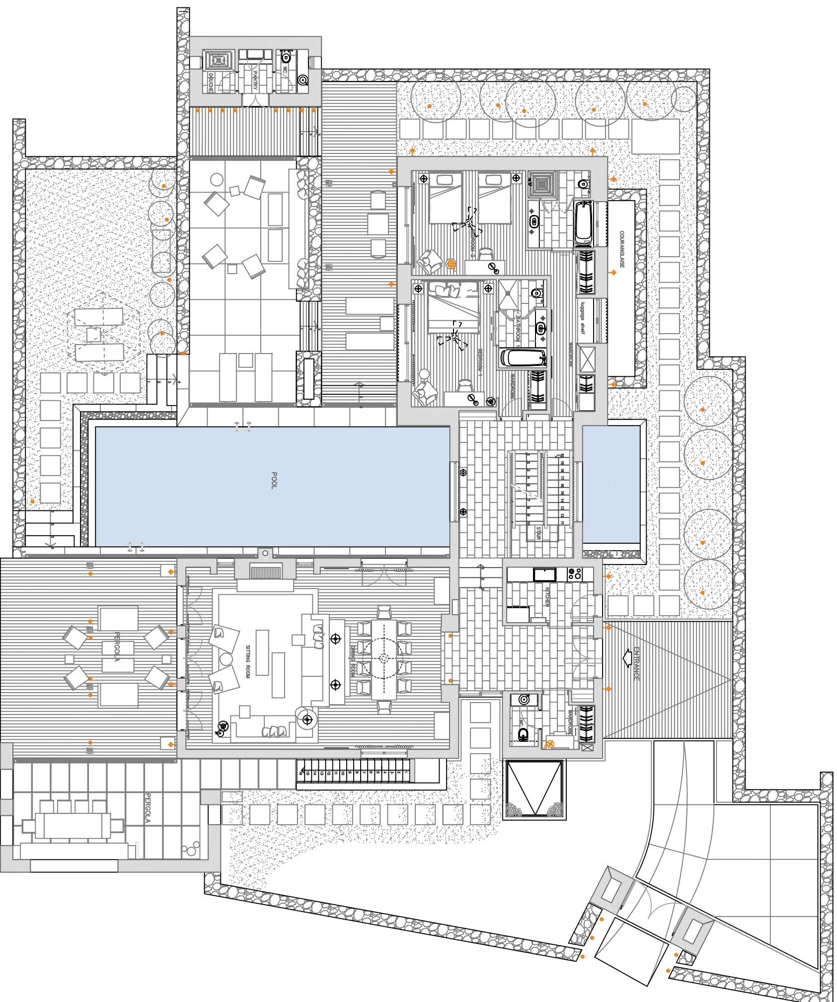
VILLA METHONI - GROUND FLOOR (SCALE 1:150 IN A3)
